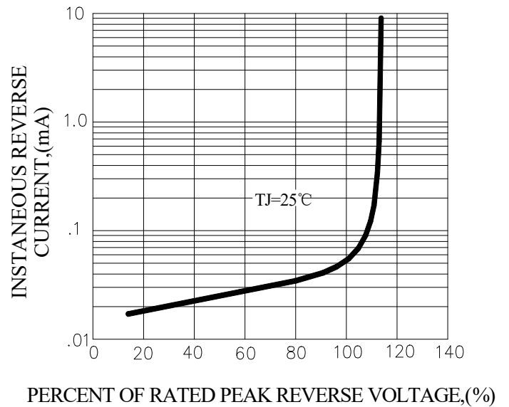
FIG.4-TYPICAL REVERSE CHARACTERISTICS
